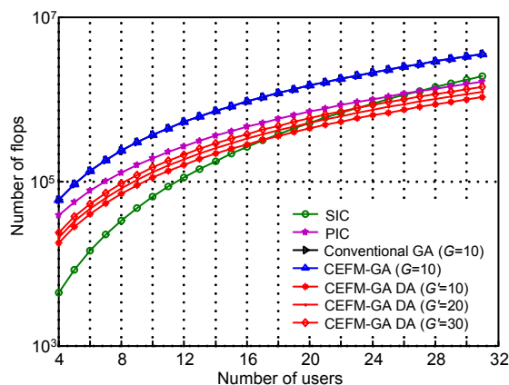
Fig. 7 Computational complexity of the proposed CEFM-GA DA compared with SIC, PIC, conventional GA, and CEFM-GA for different numbers of users
