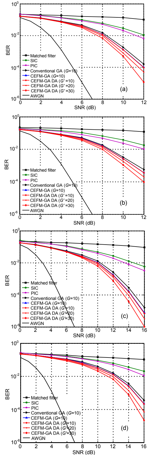
Fig. 4 BER performance of different MUDs for a lognormal fading UWB system in CM1 (a), CM2 (b), CM3 (c), and CM4 (d), where four users and a processing gain of N_s=31 are supported
